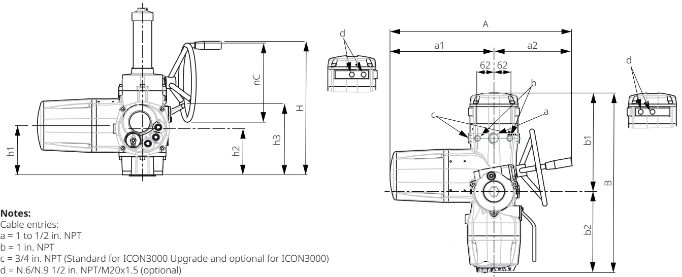
Figure 4. Optional Profibus Module with Reduced Manual Override
