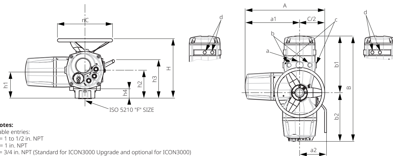
Figure 2. Optional Profibus Module with Standard Manual Override
